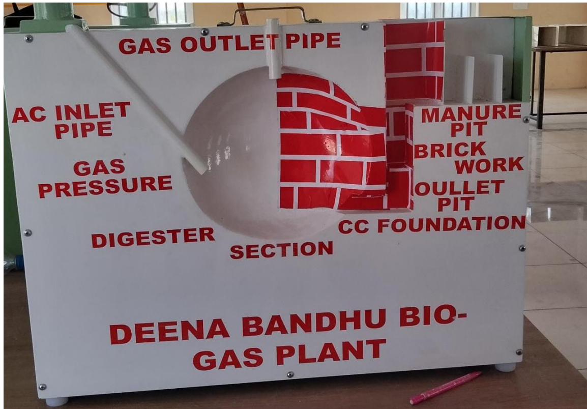
Deenabanthu Biogas plant model
