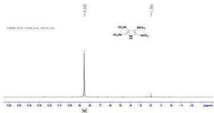
Figure 1: ^1\text{H} NMR spectrum of 2,3,4,5-tetranitropyrrole (II) in acetonitrile- d_3 .
