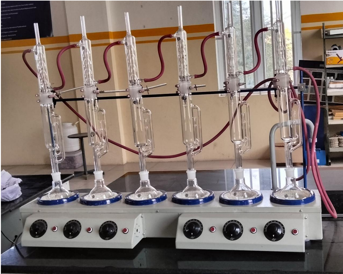
Soxhlet Apparatus
